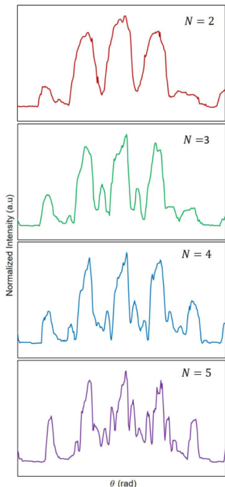
FIGURE 4. Experimental diffraction pattern with various slits number. In the experiment, the distance between the slit and the screen ( L ) is fixed, 2 m. The slit width ( d ), and the slit spacing ( b ) used are 50 and 75 \mu\text{m} , respectively. The laser used is helium laser with \lambda = 6328 \text{ \AA} .
